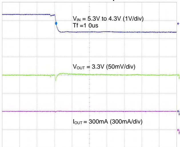
Time (50us/div)
