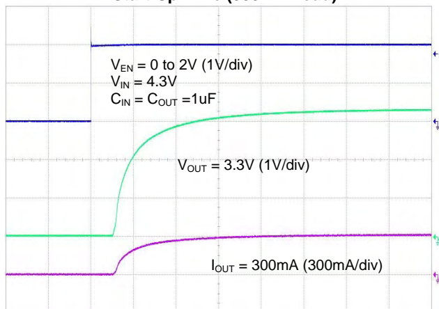
Time (50us/div)
